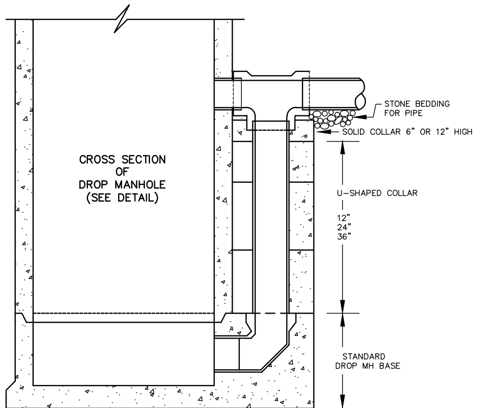
U-SHAPED COLLAR
