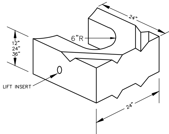
U-SHAPED COLLAR
