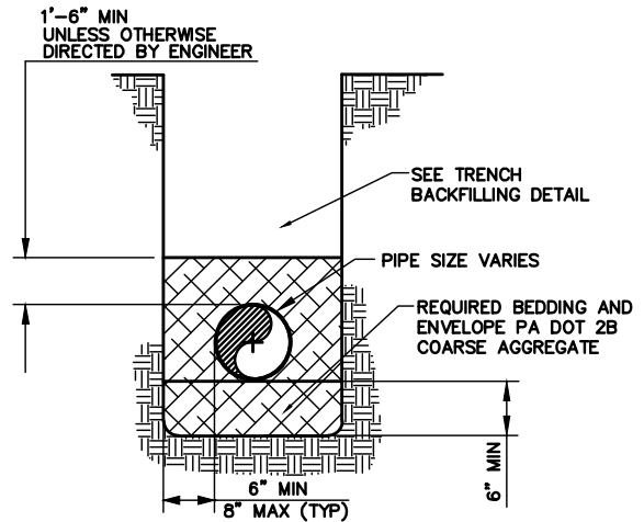
STANDARD PIPE BEDDING—SANITARY MAIN
