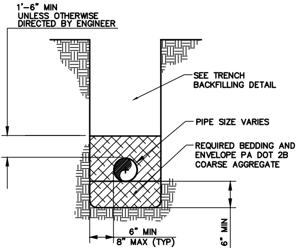
STANDARD PIPE BEDDING— SANITARY LATERAL
