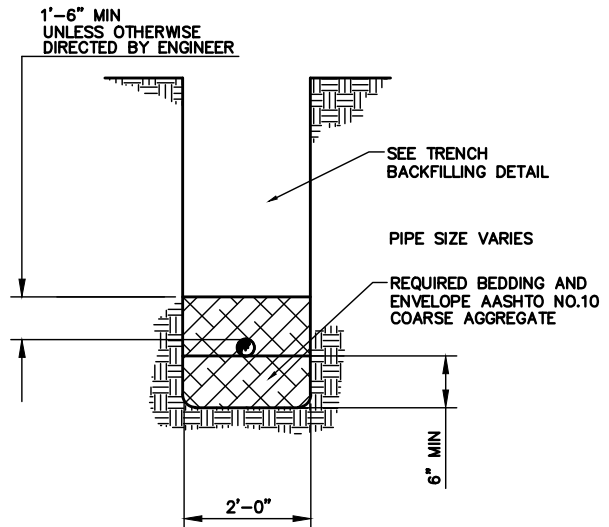
STANDARD PIPE BEDDING— WATER SERVICE
