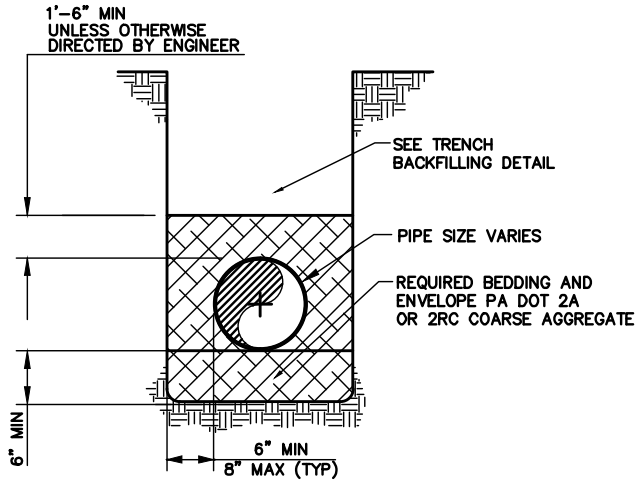
STANDARD PIPE BEDDING—WATER MAIN
