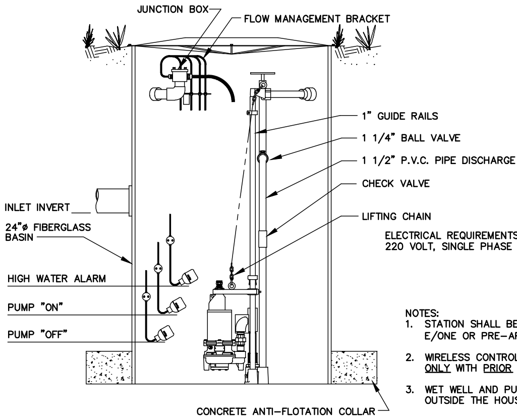
BASIN ASSEMBLY SIDE VIEW
