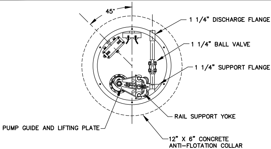
BASIN ASSEMBLY TOP VIEW
