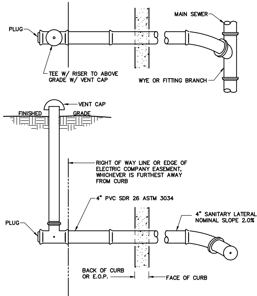
SANITARY LATERAL SHALLOW SEWER DETAIL NOT TO SCALE
