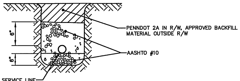
1 1/2" RESIDENTIAL SERVICE/SPRINKLER LINE CONNECTION NOT TO SCALE
