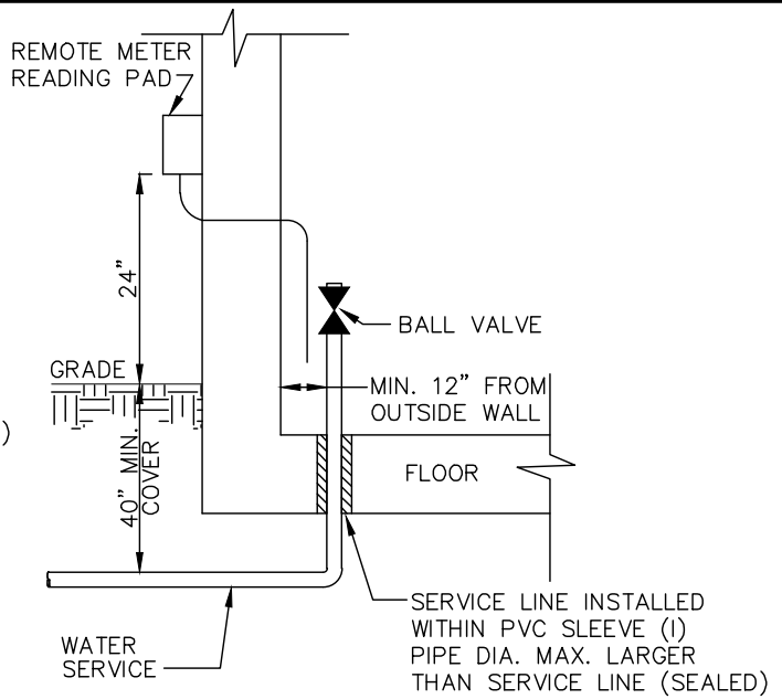
THROUGH FLOOR SERVICE
