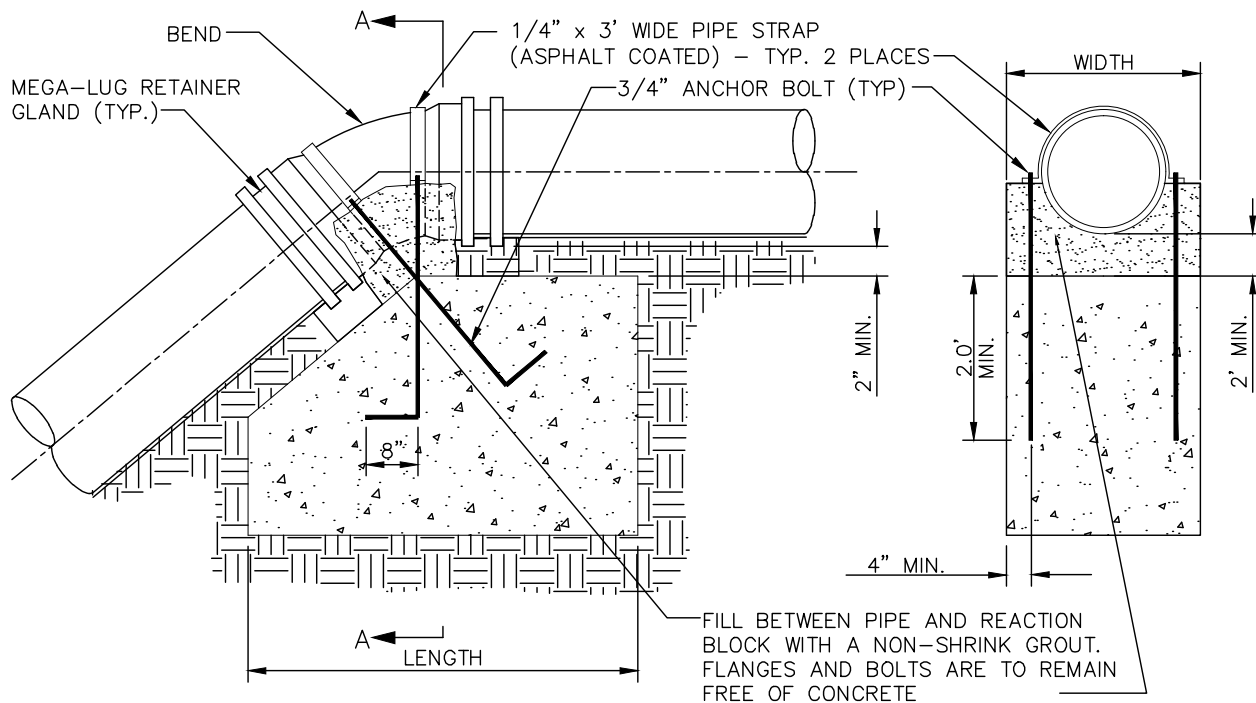
TYPICAL SECTION VERTICAL THRUST UPWARD NOT TO SCALE
